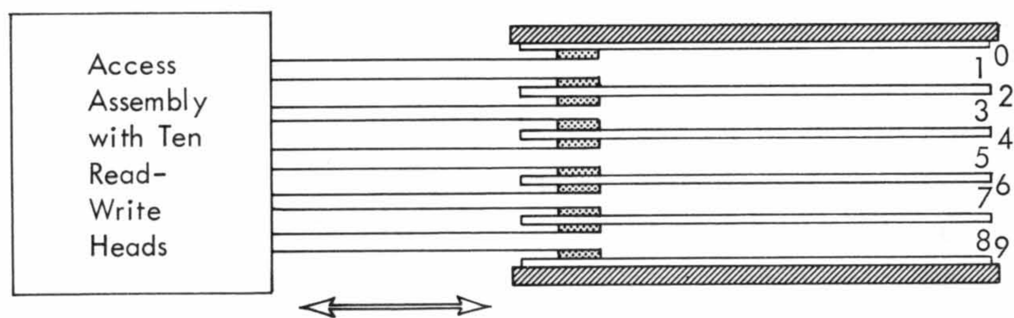
Figure 4. Access Assembly
