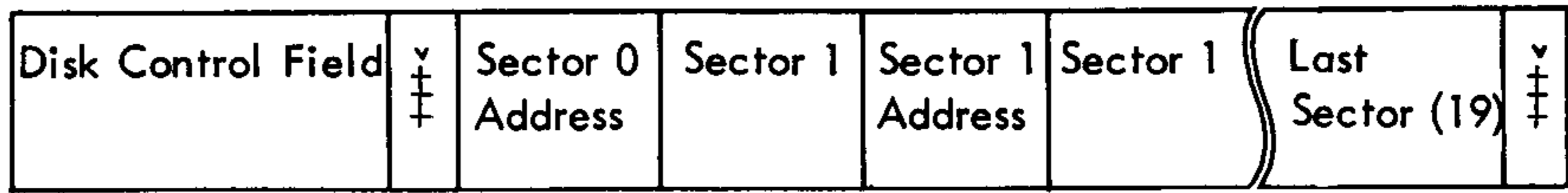
Figure 10. Core Storage Layout--Write or Read Track Sectors with Addresses
